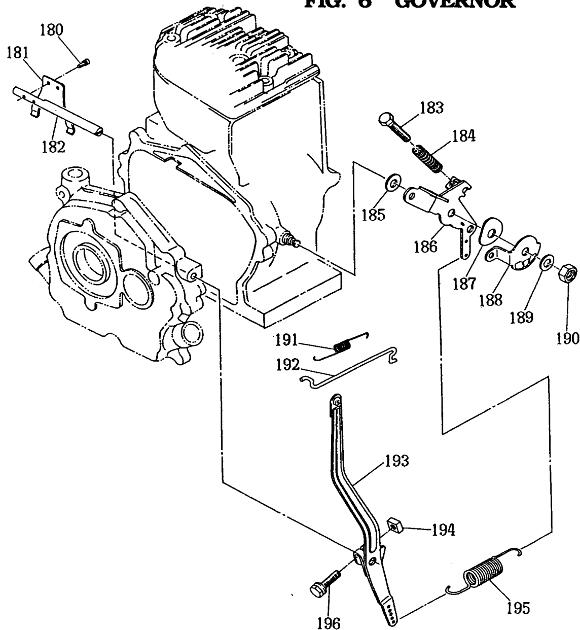
FIG. 6 GOVERNOR
