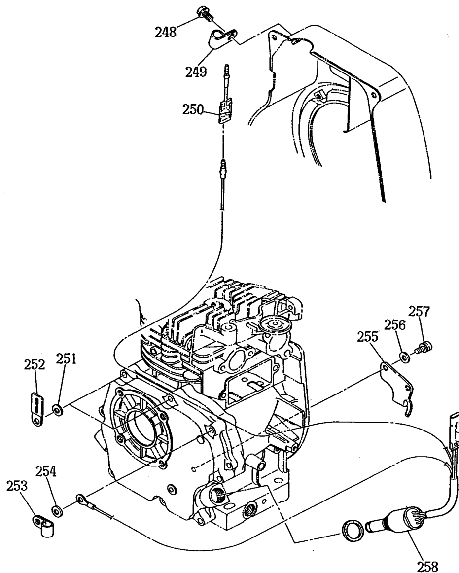
FIG. 11 OIL SENSOR
